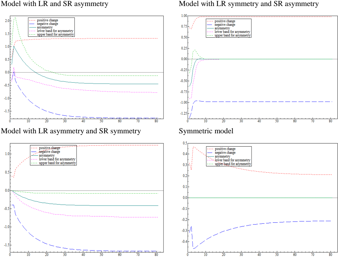
Figure 2 Cumulative asymmetric adjustments of natural gas prices
