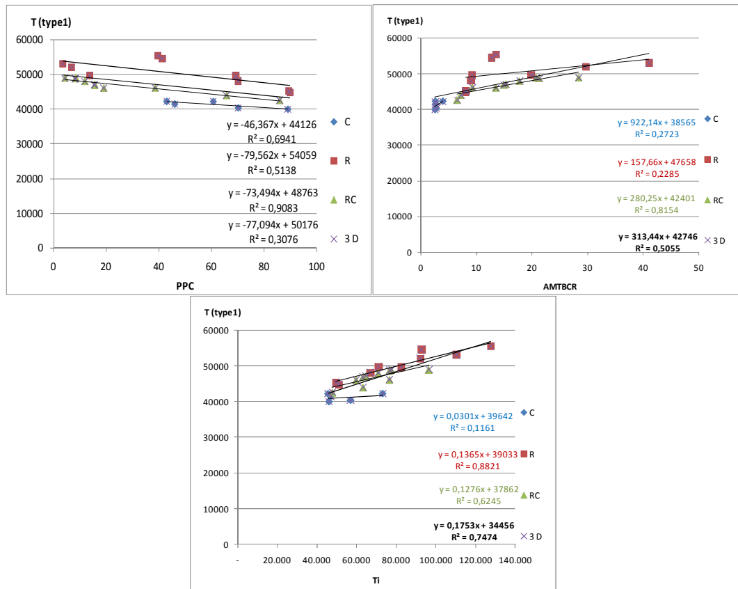
Fig. 8 – Linear regression for total travel time with PPC , AMTBCR and T_i for type 1
