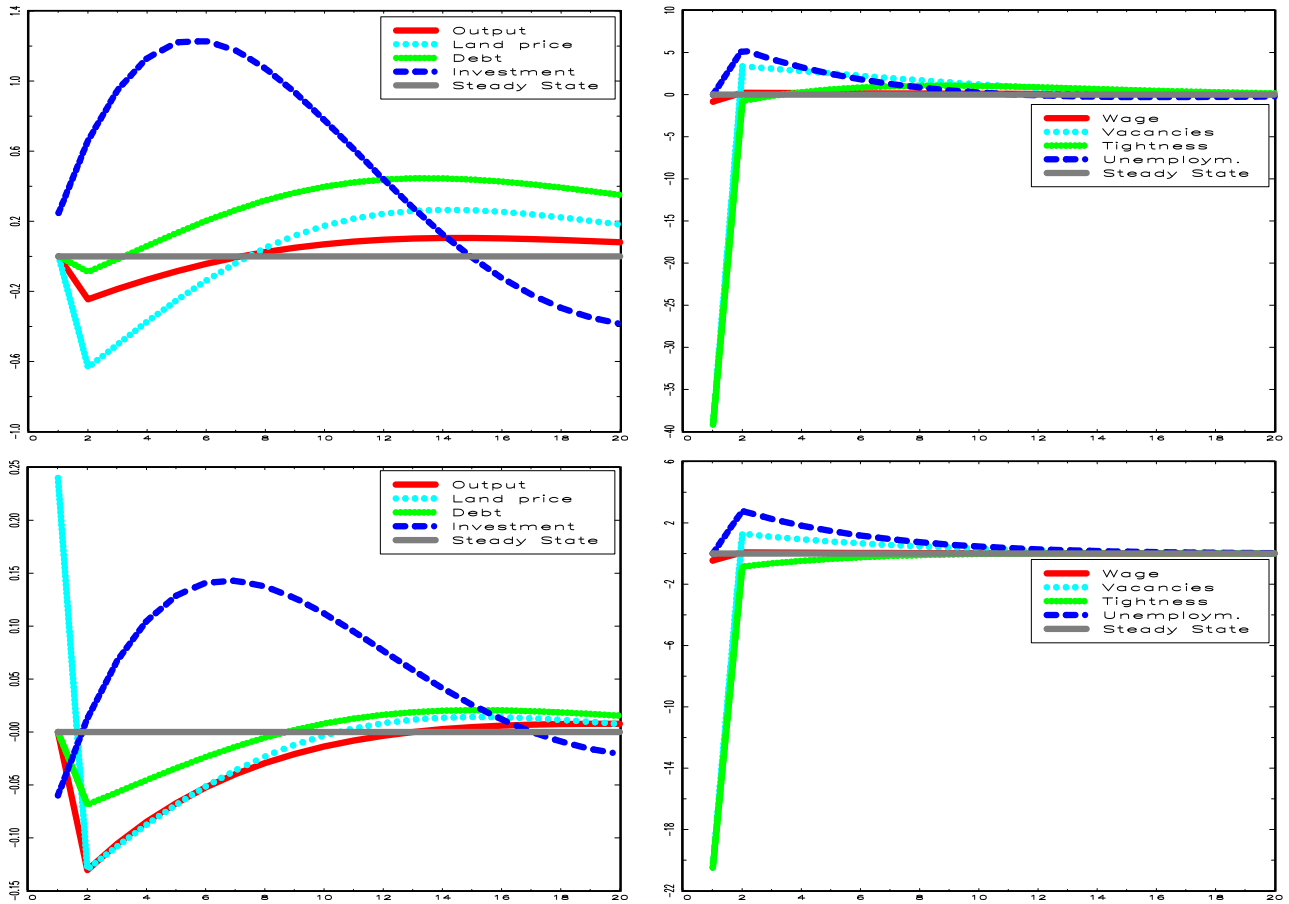
Figure 6: Impulse responses to leverage shock (top) and sunspot shock (bottom) in the indeterminate model.
