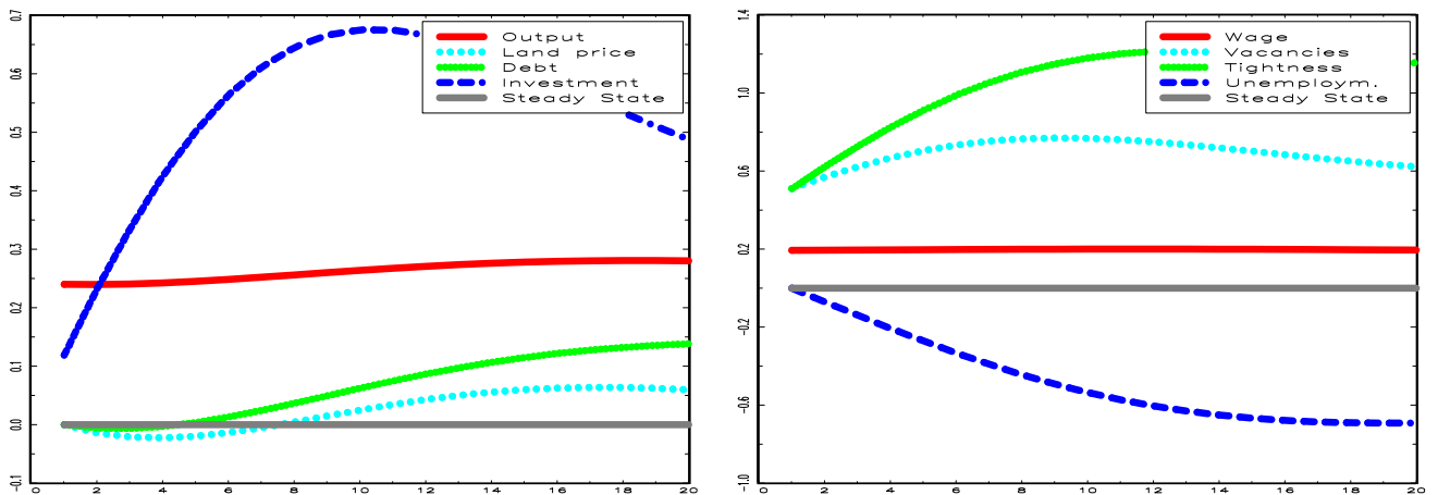
Figure 4: Impulse responses to a positive TFP shock in the indeterminate model.
