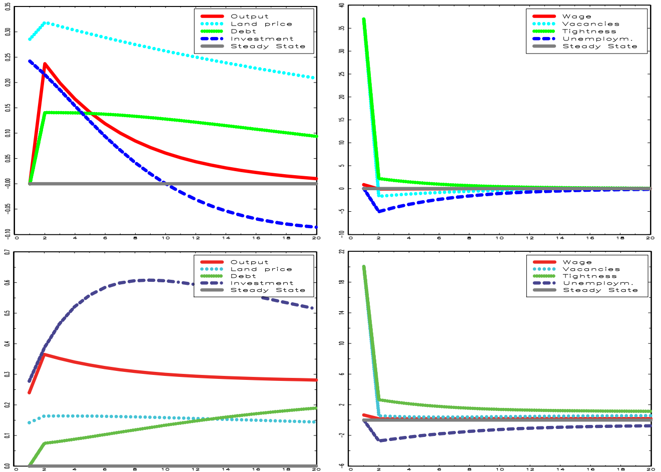
Figure 5: Impulse responses to a land price shock (top) and to a TFP shock (bottom) in the determinate model.
