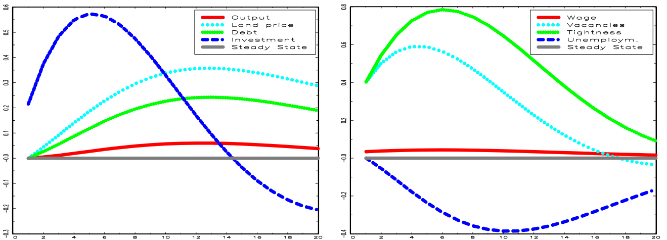
Figure 3: Impulse responses to a positive land price shock in the indeterminate model.
