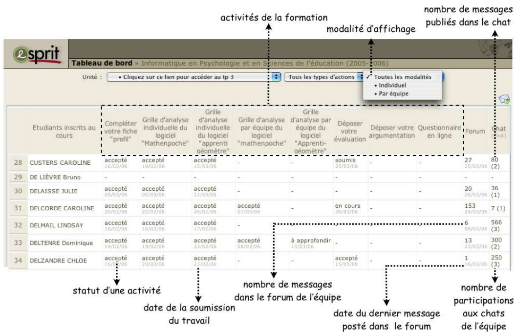
Figure 1. Dashboard
