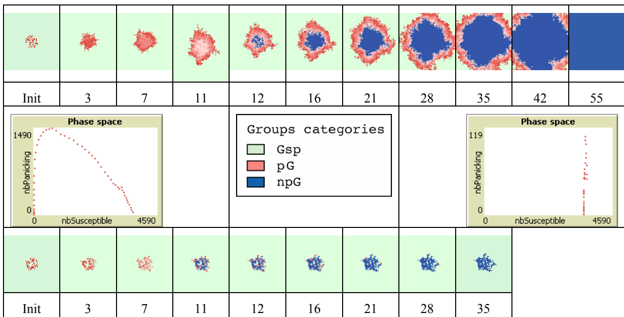
Figure 4 Phases space and screen-shoot of 2 simulations
