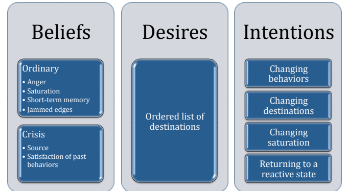
Figure 5: Beliefs, Desires and Intentions of our agents.
