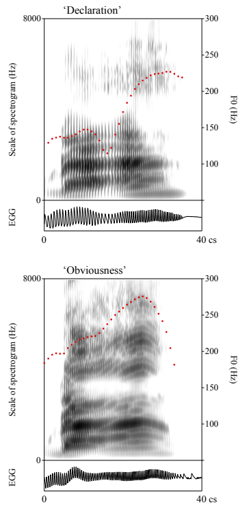
Figure 2. Spectrograms, F_0 tracings and electroglottographic signals for the Vietnamese syllable /dã C2 / under two reading conditions. Same tokens as in Figure 3.
