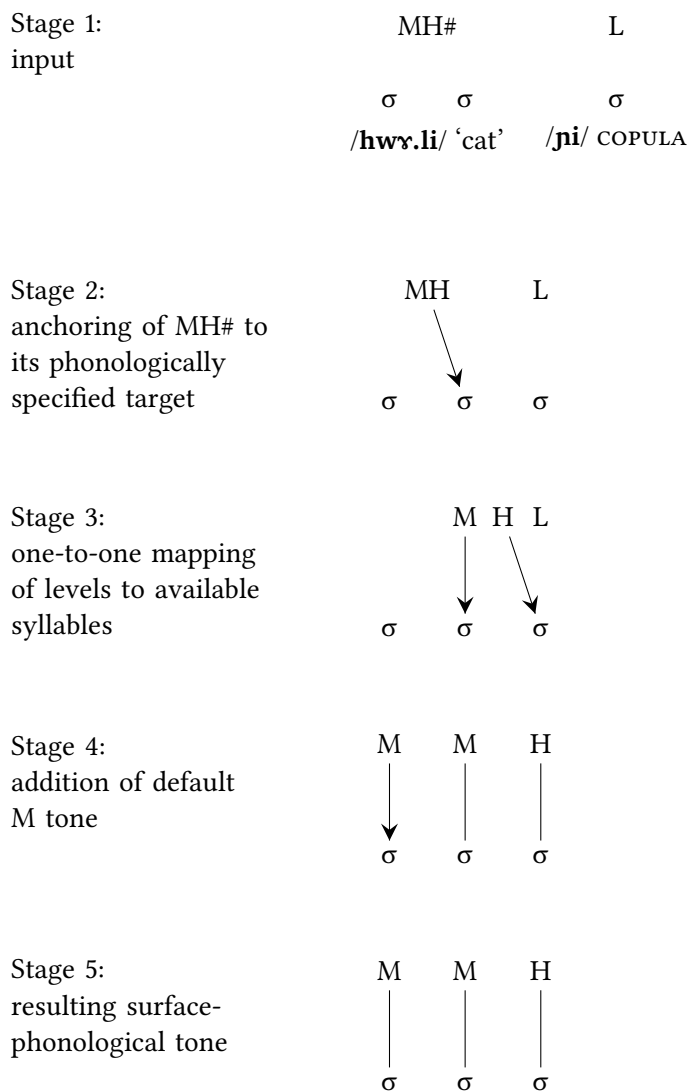
Figure 2.1: A detailed representation of tone-to-syllable association for /hwɤ.li/ 'is (a/the) cat'.
