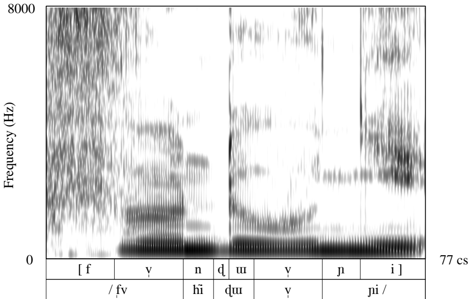
Figure 12.2: An illustration of the reduction of the relativizer /hĩ/ to a nasal consonant. Top: phonetic transcription; bottom: phonemic transcription. Speaker: F5.
