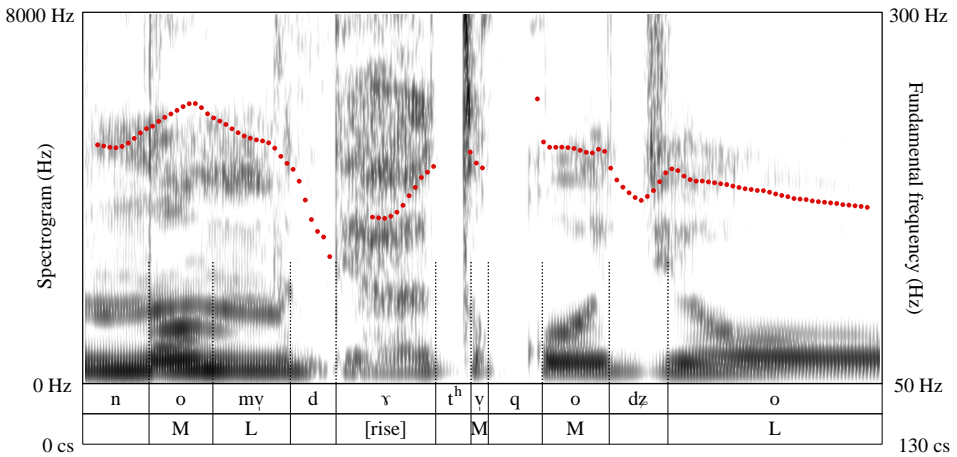
Figure 8.4: Spectrogram and F 0 curve for example (11), showing the rising realization of the syllable / ɗɿ / in / ɗɿ!-t h ɿ!qo! / ‘way over there’.
