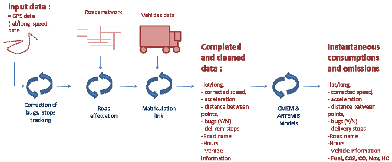
Figure 36 Calculation of fuel consumptions and pollutants emissions for non Volvo-Renault vehicles
