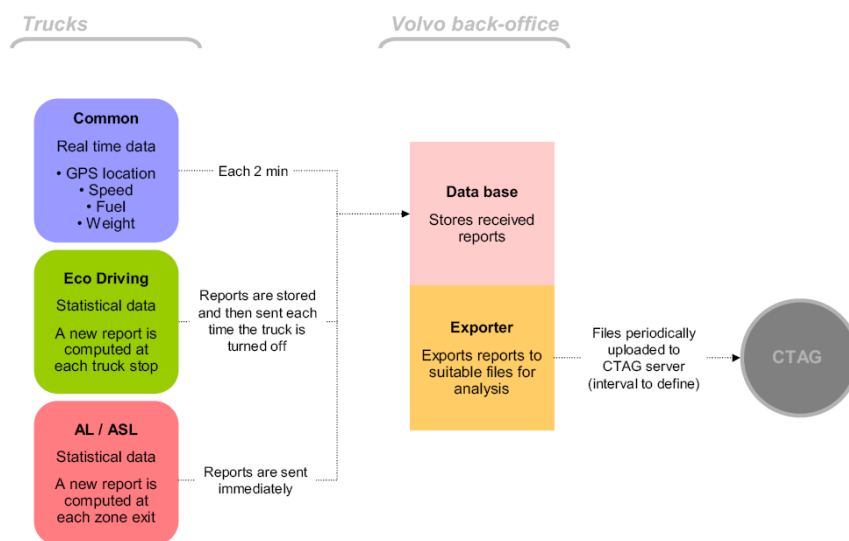
Figure 17 Data logging schema and data retrieval with Volvo systems.
