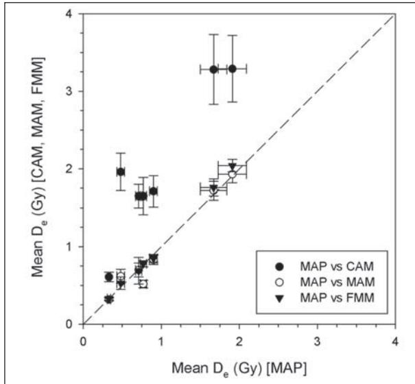
Fig. 6: Comparison of mean D_e values calculated for different statistical approaches using the Minimum Age approach of Preusser et al. (2007) as reference (MAP).
