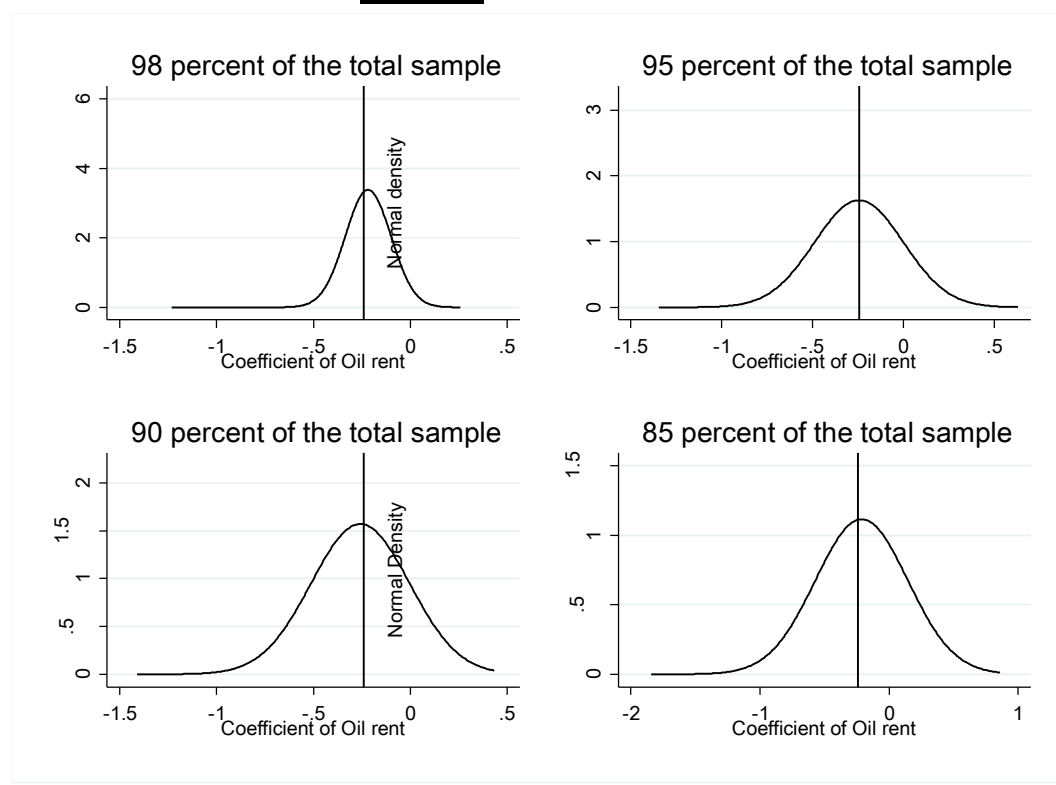
Figure 5: Robustness check
