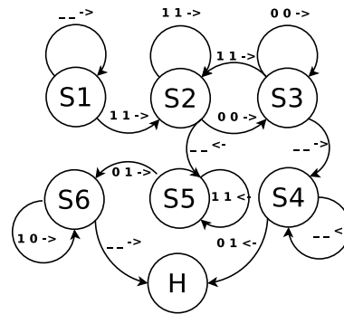
Figure 1: Generative grammar of Binary Number System
