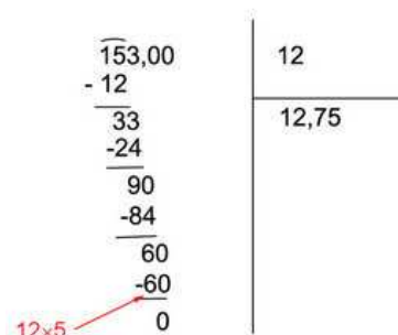
Figure 4: Hand division in Hindu-Arabic system
