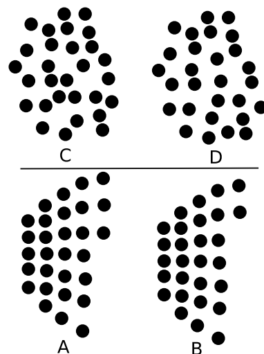
Figure 5: Cardinality vs structural properties (Card(A) = Card(C), Card(B) = Card(D) and Card(A) - Card(B) = Card(C) - Card(D) = 1)
