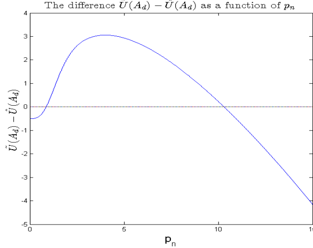
Figure 3: The graph of (\tilde{U} - \hat{U}) as a function of p_n
