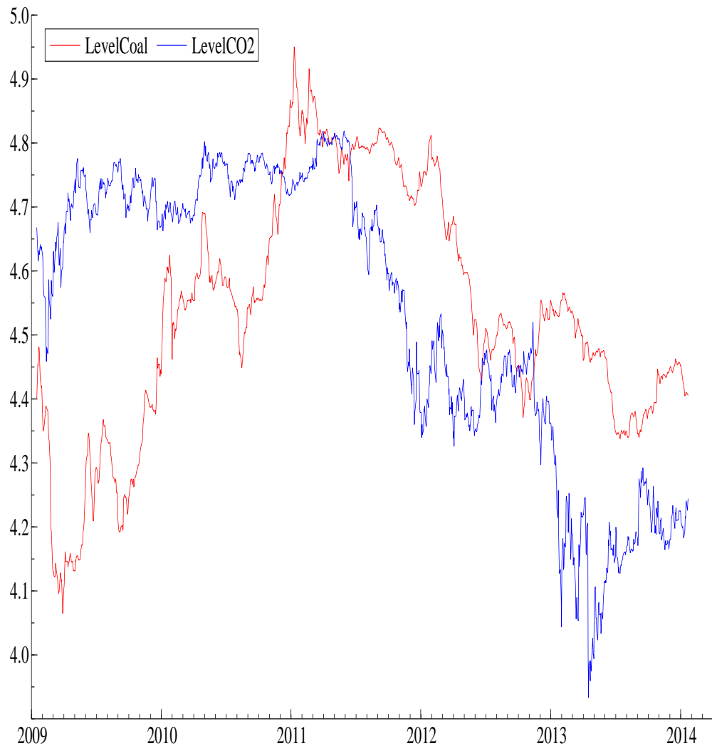
Figure 4: Common levels between the Coal and CO_2 emissions after mid-2011
