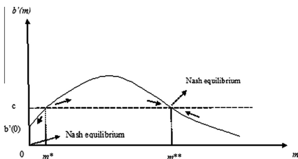
Figure 2. Coordination equilibrium in the presence of two thresholds.
