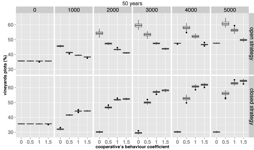
Figure 6: Percent of coverage on potential areas of vineyards plots in the landscape after 50 years of simulations of climate change and different cooperative policies. Organization of graphs as in Figure 5.
