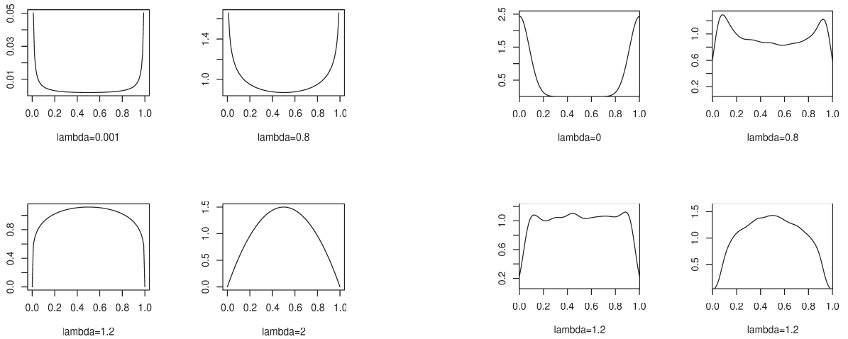
Figure 9: Invariant density function of the Wright-Fisher diffusion with mutations for different values of \lambda (left part) and empirical distribution (using 1000 independent Monte Carlo simulations) of X_{100000}^1 in the Markov chain market game with parameters a = 0.1 and b = \lambda a^2 (right part).
