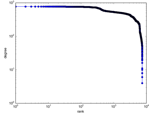
(a) Recurrence Plot of the inter-sector recurrence matrix. (b) Degree rank plot of the inter-sector recurrence network.
