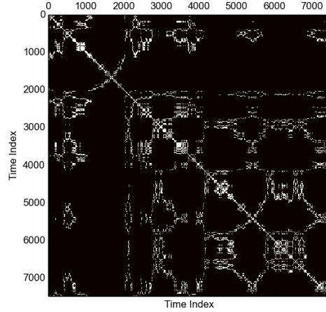
(a) Recurrence Plot of the inter-sector recurrence matrix. (b) Degree rank plot of the inter-sector recurrence network.
