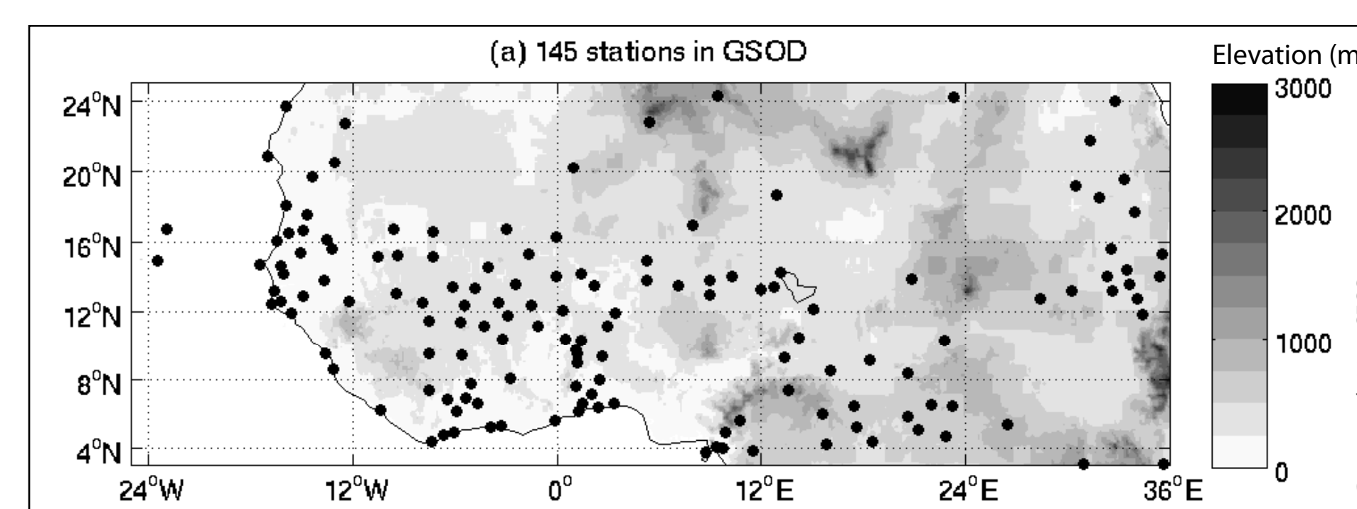
Figure 1. Meteorological data network available in West Africa: location of the 145 stations available in GSOD having at least 3650 daily entries in the 1973-2013 period.
