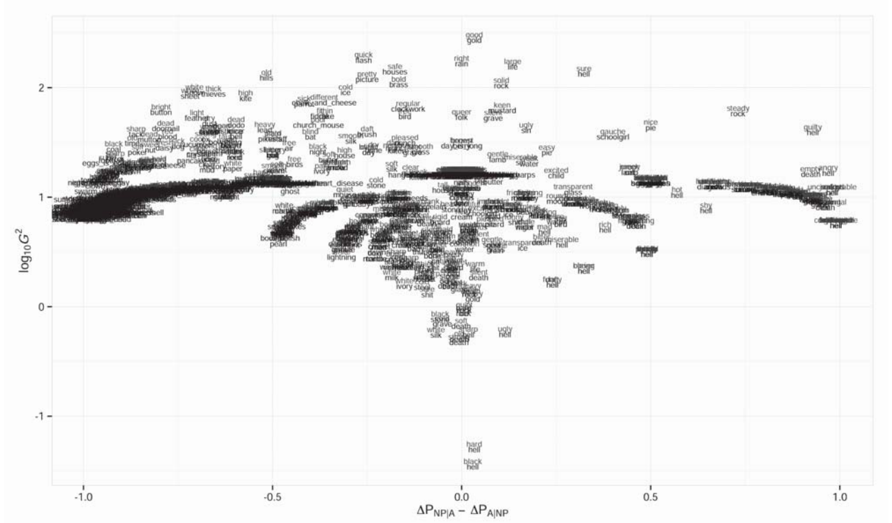
Figure 3: Distribution of A-NP pairs according to \Delta P differences ( x -axis) and log-likelihood ratio ( y -axis, logged)
