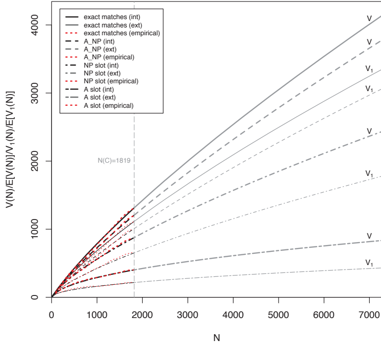
Figure 1: Vocabulary growth curves for exact A as NP matches, concatenated slots (A_NP), the A slot, and the NP slot with LNRE interpolations (int) and extrapolations (ext) to four times the sample size
