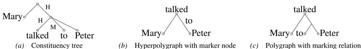
Figure 10: Ternary grouping
