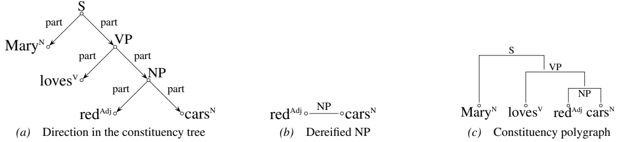
Figure 3: Dereification of constituency trees
