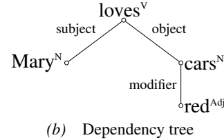
Figure 1: Constituency and dependency trees
