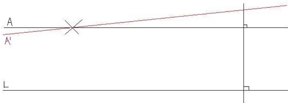
Figure n°1 – Euclidean postulate n. 5 (the parallel postulate)
