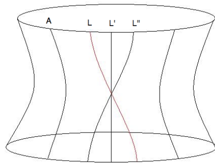
Figure 3 – Representation of parallel lines L, L' and L'' passing through the same point
