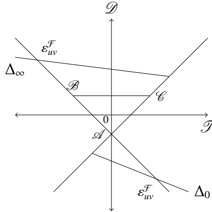
Figure 5: Flip bifurcation.
