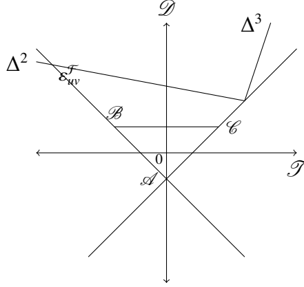
Figure 3: Flip bifurcation with under-accumulation of capital.
