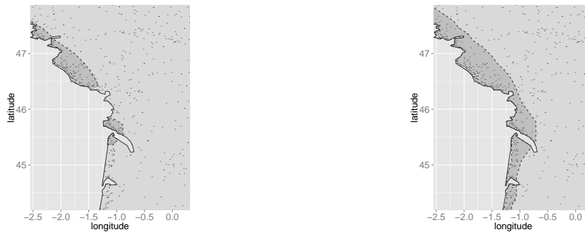
FIGURE 20. Convex hull of hot spot areas (zoom on the Atlantic coast), without border correction (on the left) and with Ripley's correction (on the right).
