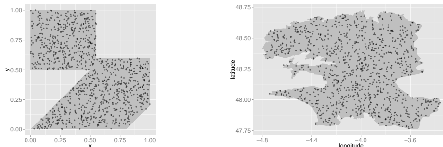
FIGURE 6. Polygon \mathcal{S} on the left and the Finistère region on the right, where 1,000 points are uniformly drawn.
