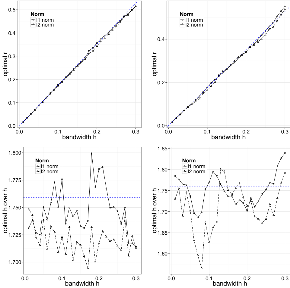
FIGURE 7. Optimal r^*(h) as a function of h on the polygon shape (on the left) and the Finistère region (on the right), from Figure 6, on top, and below, ratio of r^*(h) over h , as a function of h .
