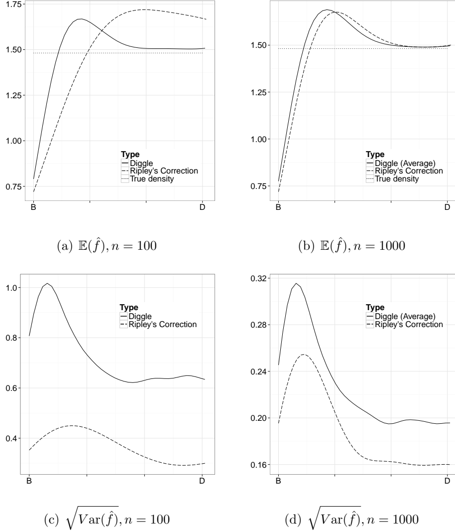
FIGURE 8. Estimation of the density in the upper left corner of polygon \mathcal{S} , on interval [B, D] , with n = 100 and n = 1,000 points, on the left and on the right, respectively, with the average density (on 1,000 samples), and the standard deviation.
