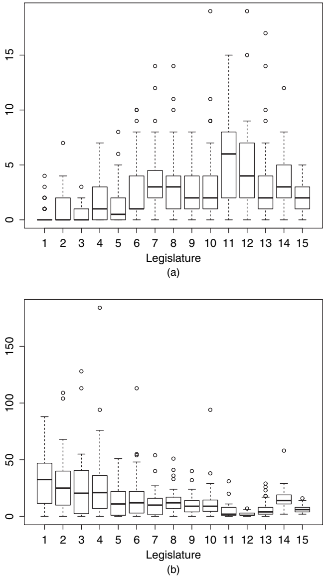
Fig. 1. Distribution of (a) executive decrees and (b) ordinary laws during the 15 legislatures of the Italian Republic
