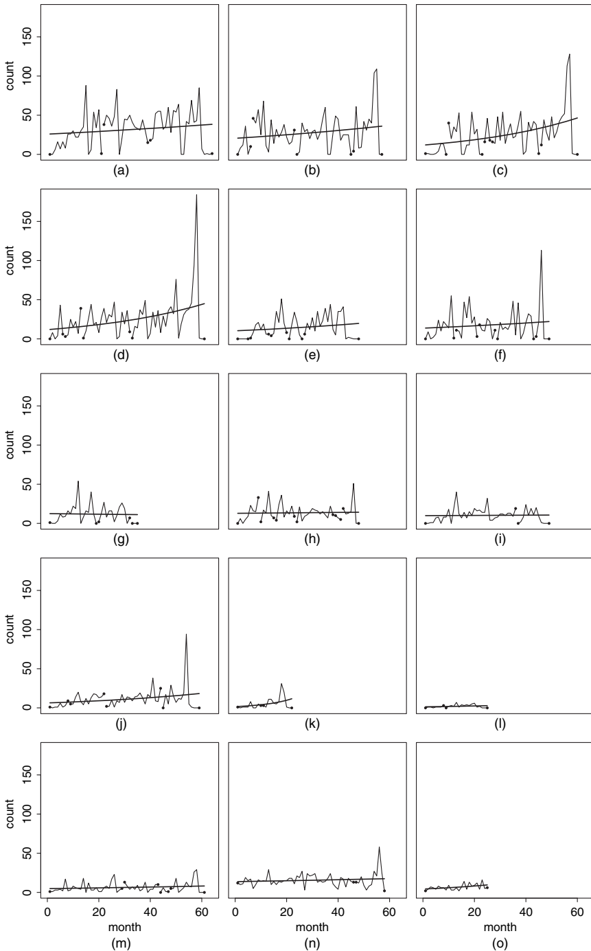
Fig. 3. Monthly counts of laws, approved in Italy under 52 governments, during 15 legislatures (the x-axis indicates the time since the beginning of the legislature; ●, appointment and resignation of each government): (a) legislature 1; (b) legislature 2; (c) legislature 3; (d) legislature 4; (e) legislature 5; (f) legislature 6; (g) legislature 7; (h) legislature 8; (i) legislature 9; (j) legislature 10; (k) legislature 11; (l) legislature 12; (m) legislature 13; (n) legislature 14; (o) legislature 15
