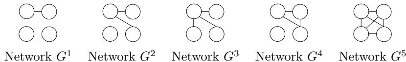
Figure 5: Some specific networks
