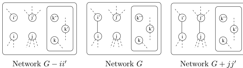
Figure 2: Intuition behind Proposition 1
