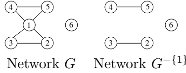
Figure 4: An interlinked star which is not a NSG
