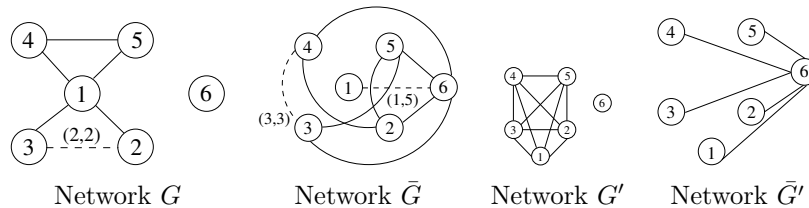
Figure 3: Networks G , \bar{G} , G' and \bar{G}'
