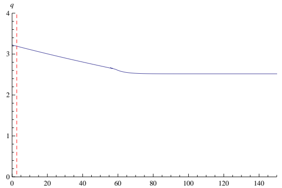
Figure 4.3: The transition inter regime: the Tobin's q
