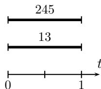
Figure 3: The unique optimal timetable
