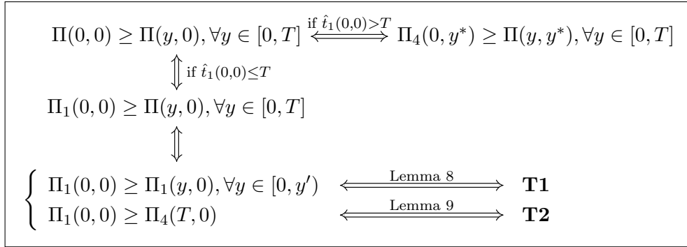
Figure 6: Structure of the proof for Proposition 6.
