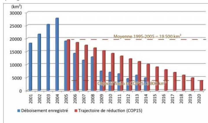
Figure 8: The reduction of deforestation since 2001 and the COP15 Brazilian pledge
