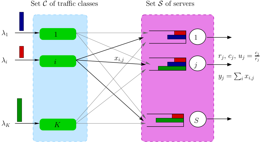
Fig. 1. Non-cooperative load balancing: each dispatcher controls a portion of the total traffic intensity and probabilistically routes its jobs so as to minimize their own mean processing cost.
