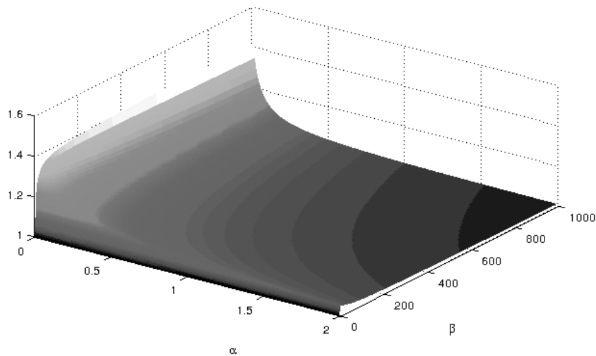
Fig. 4. Evolution of the inefficiency as a function of \alpha and \beta for K = 5 dispatchers and S = 1000 servers.
