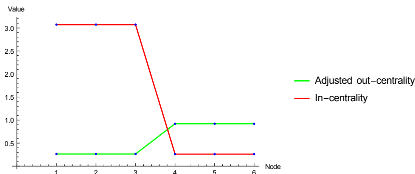
Figure 10: Graphical representation of the in-centrality profile and the profile of adjusted outcentrality for the 6 firms of the economy, \alpha = 0.9
