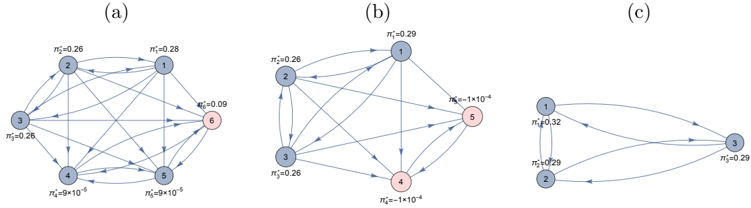
Figure 11: The firm dynamics triggered by the initial elimination of Firm 6 (a), followed by the consecutive step (b) where Firms 4 and 5 incur losses (i.e. obtain negative profits) and are eliminated. In the resulting network (c) all firms make positive net profit
