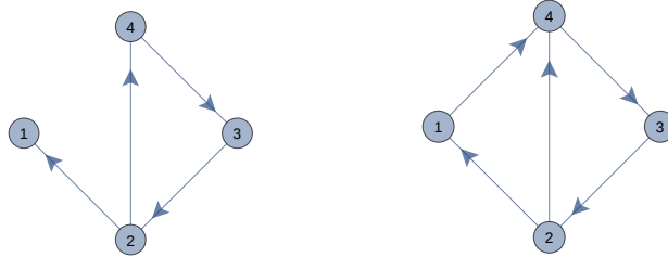
Figure 8: Two different production networks, whose only difference concerns the existence, or not, of the link from node 1 to node 4. All nodes/firms are supposed to produce a consumption good with equal preference weights.
