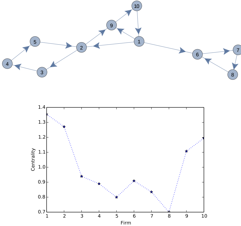
Figure 5: A production network in the upper panel, with the corresponding profile of Bonacich centralities for each of the nodes displayed in the lower panel.
