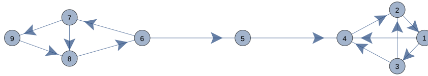
Figure 2: A simple production network illustrating the discussion included in Example 1.
