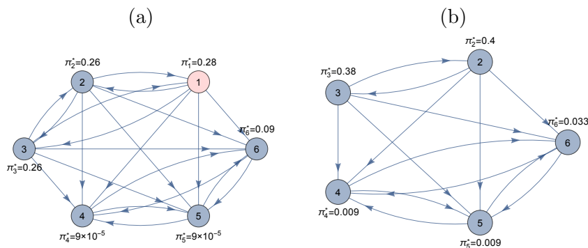
Figure 12: The elimination of Firm 1 (a) does not cause thereafter the exit of any other firm from the network.
