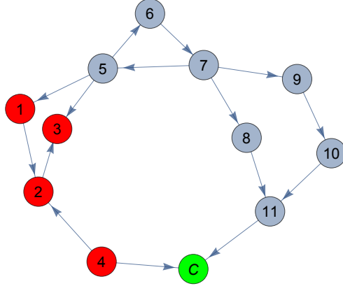
Figure 1: An extended production network \hat{G} that includes the consumer node. The blue nodes are those that satisfy conditions (a)-(b) in Proposition 1, while the red ones do not. The green node represents the consumer demand.
