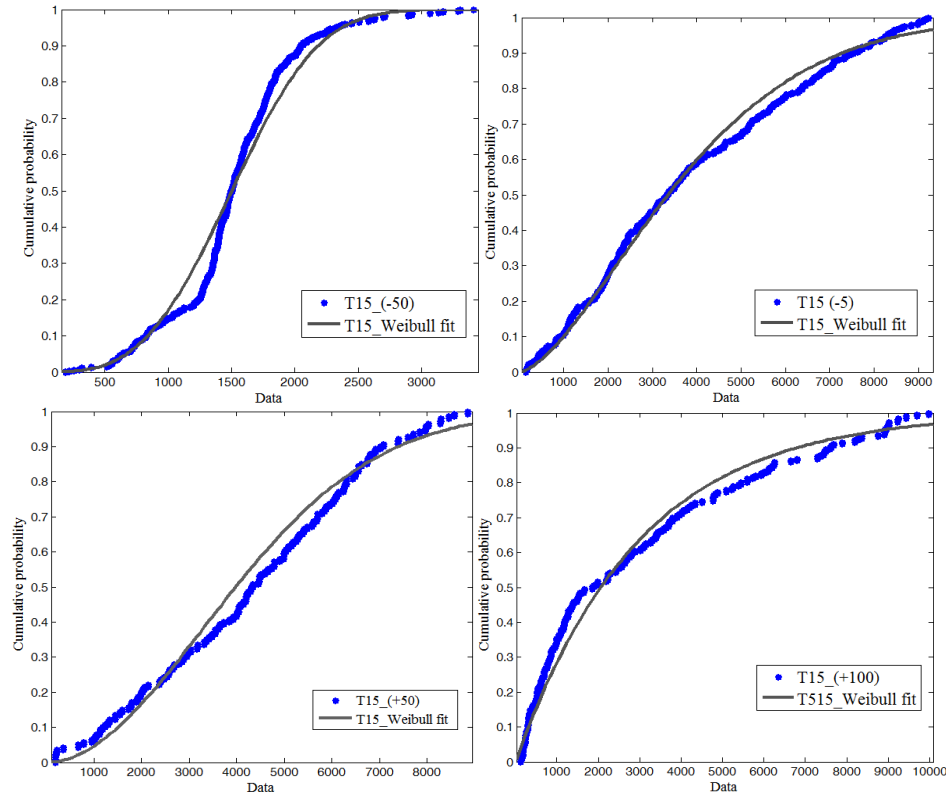
Figure 2. Cumulative probability plot and fitted Weibull distribution for the sections S -50 , S -5 , S +50 , S +100 .
