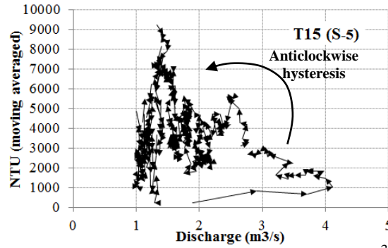
Figure 3. Example of temporal dynamic between flow discharge ( \text{m}^3/\text{s} ) and associated turbidity (NTU) in S-5.
