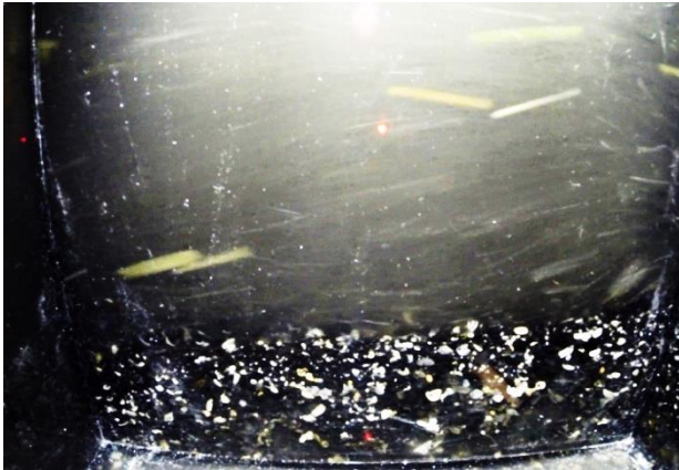
Fig. 9 Snapshot from video camera situated on a negative slope invert at 50 m from the gate after one minute since the flush beginning
