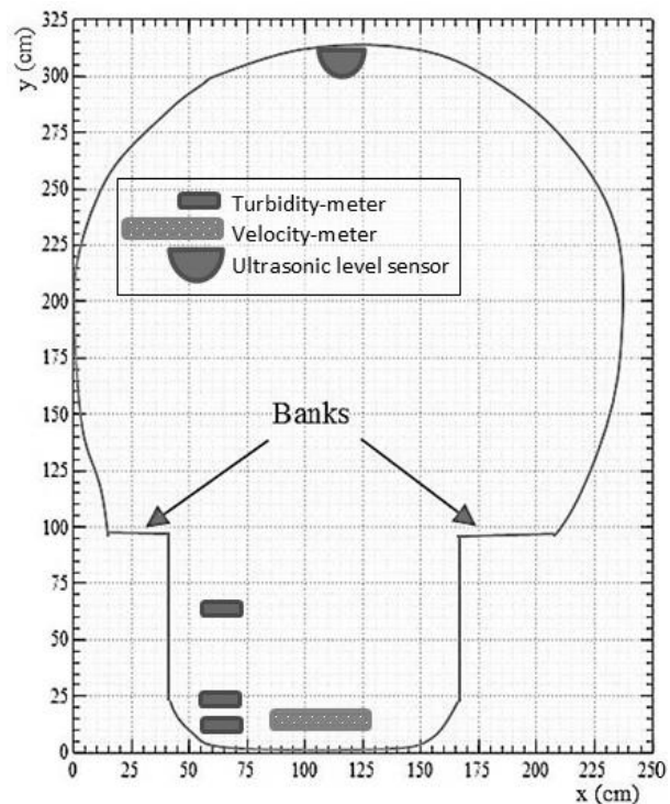
Fig. 1 Sewer Cross-section Details and Measurement Equipment Position
