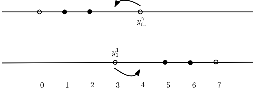
Figure 7: v_1^c = y_1^1 ; an FIP is possible
