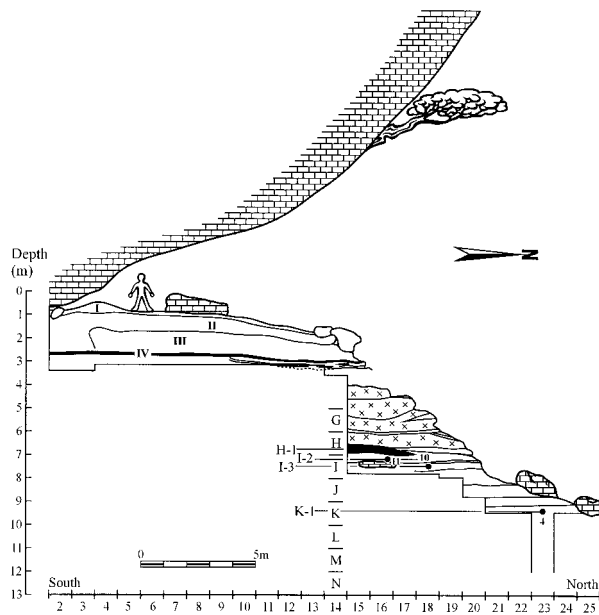
Fig. 1. Stratigraphic profile of the Bau de l'Aubesier. The positions of the Aubesier 4, 10, and 11 are indicated, as well as the H-1 black combustion horizon.
