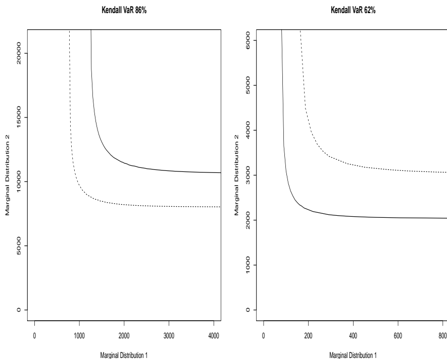
Figure 11: This figure represents the Kendall VaR obtained using a Gumbel copula with two different lognormal marginal distributions. The figure on the left compares the 86% Kendall VaR to its lower-orthant equivalent. We observe that the Kendall VaR is inferior to the lower-orthant one. The figure on the right compares the 62% Kendall VaR to the upper-orthant VaR computed from the survival copula of the Gumbel. Here, we see that the Kendall VaR is superior to the upper-orthant one.
