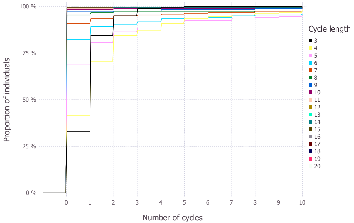
Figure 5: CDF of Strict UCR cycle lengths in the consumption data (for length <20) for observed demands when Strict UCR contains cycles.
