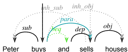
Figure 3: Shared dependents
