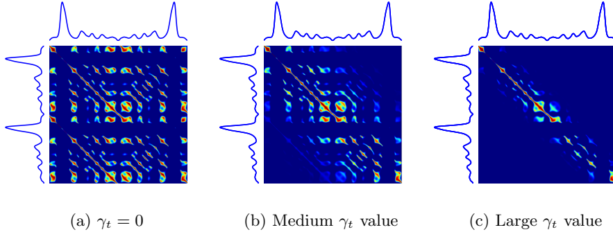
Fig. 1: Impact of the k_{t\text{RBF}} kernel on similarity matrices A^{1,2} . From left to right, growing \gamma_t values are used from \gamma_t = 0 ( i.e. the k_{\text{RBF}} kernel case) to a large \gamma_t value that ignores almost all non-diagonal matches. Blue colors indicate low similarity whereas red colors represent high similarity. 1 Best viewed in color.
