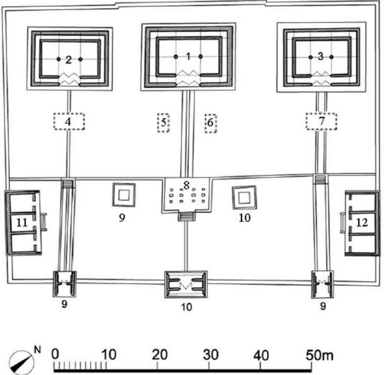
Fig. 12. Plan of the Three Temples complex, Erdeni juu (Brandt and Gutschow 2003) 1. Central Temple; 2. Right Temple; 3. Left Temple; 4. Temple to the Mahārājas; 5. Shrine to Avalokiteśvara; 6. Shrine to Maitreya; 7. Temple to the Mahārājas; 8. Ceremonial archway; 9. Tomb of Abadai Khan; 10. Tomb of Fombodorji; 11. Amītāyus Temple; 12. Camba[γarbu]/Tshangs pa dkar po Temple; 13. Entrance Gate
