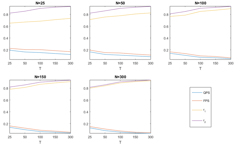
Figure 5: Quality of state identification: filtered probability of recession
