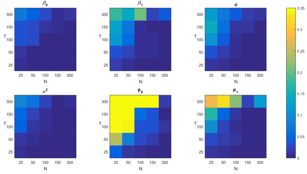
Figure 1: Kullback-Leibler distance between \hat{\theta}_i(\hat{f}) and \hat{\theta}_i(f) , with \theta = (\beta_0, \beta_1, \phi, \sigma^2, p_0, p_1)
