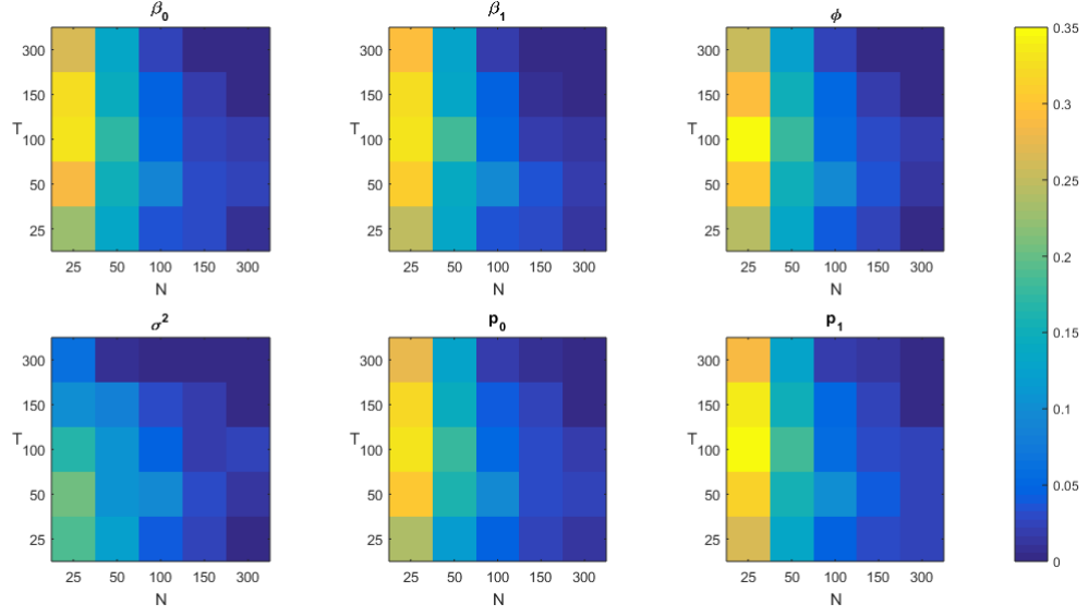
Figure 2: Kullback-Leibler distance between \hat{\theta}_i(\hat{f}) and \hat{\theta}_i(f) , with \theta = (\beta_0, \beta_1, \phi, \sigma^2, p_0, p_1) , aberrant replications excluded
