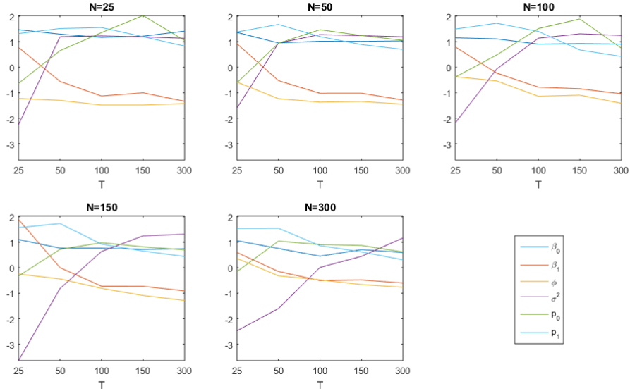
Figure E.1: Skewness of the t-statistics corresponding to the estimates \hat{\theta}_i(\hat{f}) at different N and T
