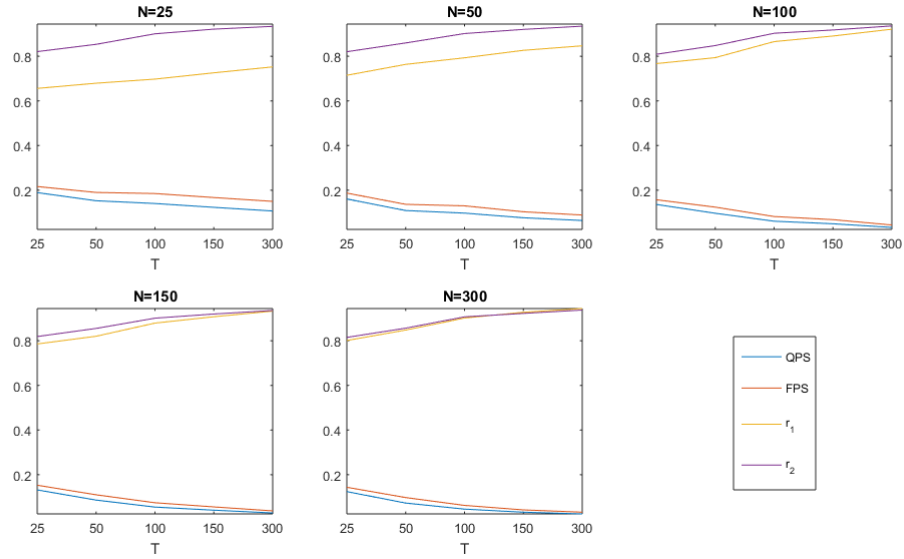
Figure 6: Quality of state identification: smoothed probability of recession
