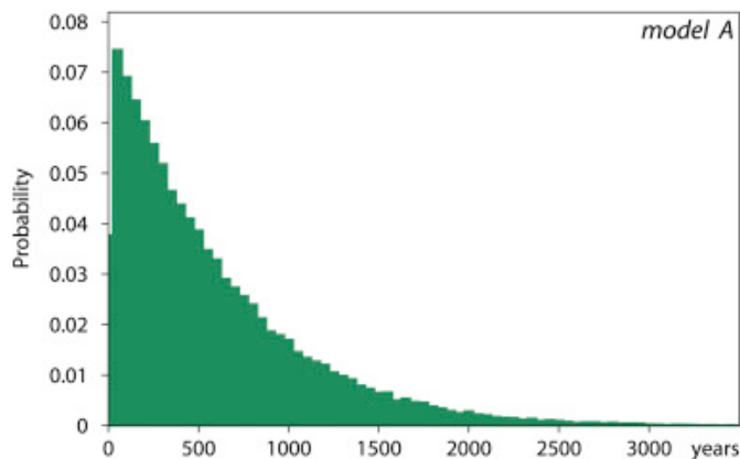
SOM Figure S8. Model A. Posterior probability distribution for the time elapsed from the end of C to the beginning of B occupations.
