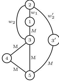
Figure 10: C = \{1, e_1, 2, e_2, 3, e_3, 4, e_4, 5, e_5, 3, e_6, 1\} , C' = \{1, e_1, 2, e'_2, 3', e'_3, 5, e_5, 3, e_6, 1\} with w_1 < w_2 = w'_2 < M but C is not a simple cycle.
