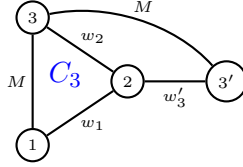
Figure 24: E_1 = \{e_1, e_2, e'_3\} , \sigma(N) = w_1 = w_2 = w'_3 < M .
