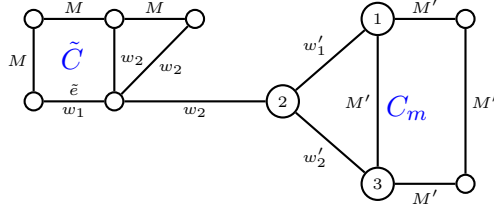
Figure 21: E_1 = \{\tilde{e}\} , w(\tilde{e}) = w_1 < w_2 \leq M in \tilde{C} and w'_1 = w'_2 < M' in C_m .
