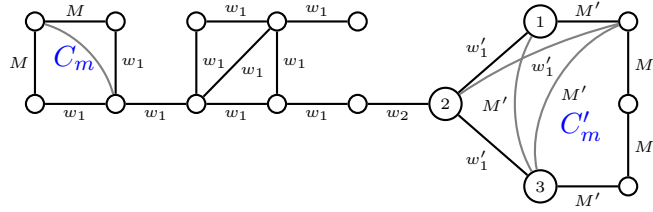
Figure 22: |E_1| \geq 2 , \sigma(N) = w_1 < M , and w_1 \leq w_2 < w'_1 = w'_2 < M' .
