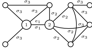
Figure 27: \sigma_1 < \sigma_2 < \sigma_3 .
