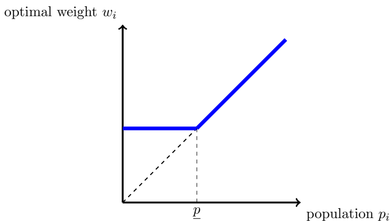
Figure 1: Optimal voting weights in the model of apportionment
