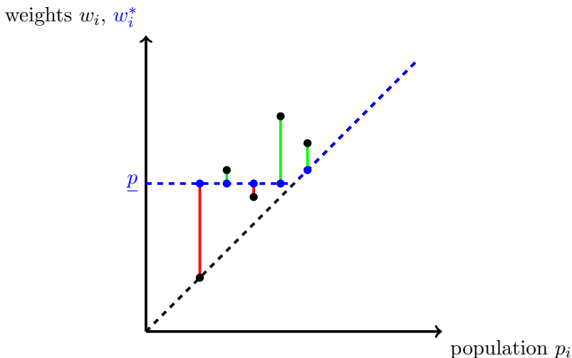
Figure 3: Definition of \underline{p} (total red length=total green length)
