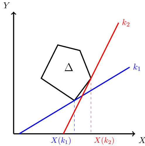
Figure 4: Solutions of (\mathcal{D}^{k_1})' and (\mathcal{D}^{k_2})' for k_2 > k_1 .
