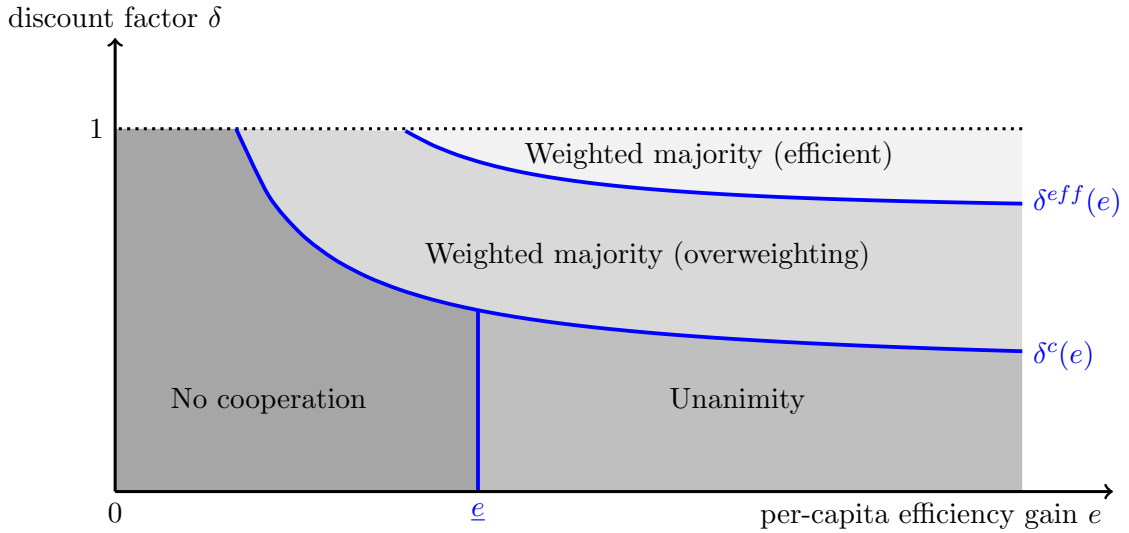
Figure 2: Optimal self-enforcing rule in the model of apportionment
