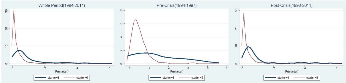
Figure G.1: Density Distribution of Propensity Score
