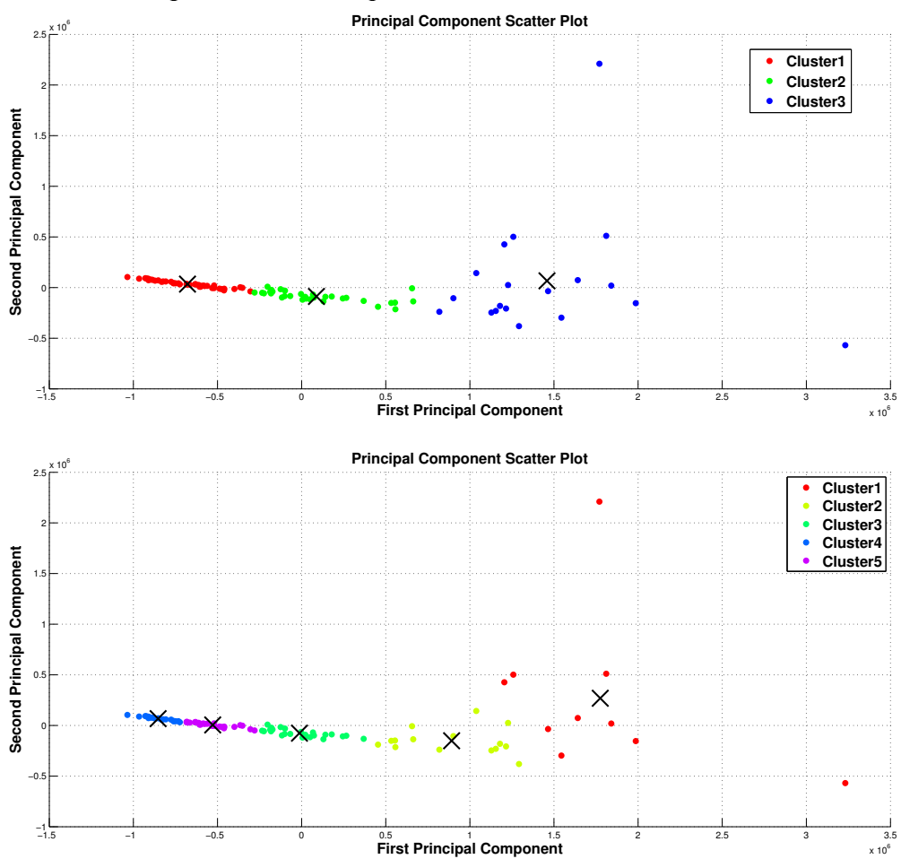
Figure 6: Cluster segmentation for K = 3 and K = 5
