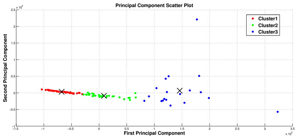
Figure 6: Cluster segmentation for K = 3 and K = 5
